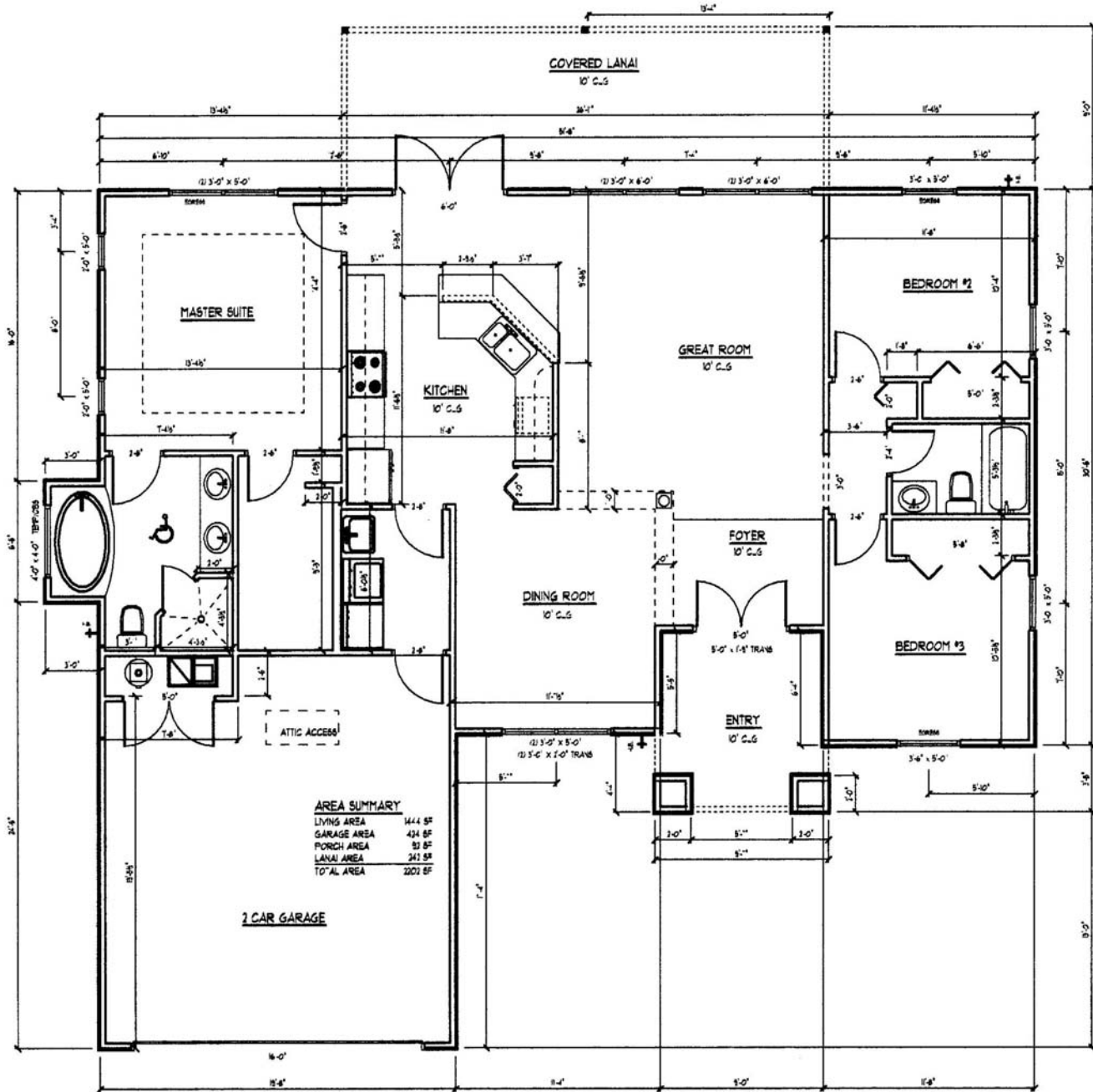
FLOOR PLAN
